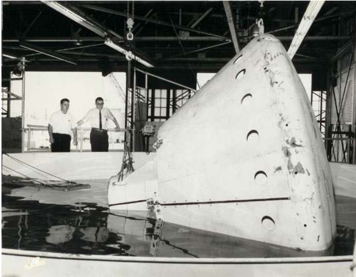
Apollo BP-25 during static stability measurement in water tank test at Ellington AFB Hangar-135 in October 1964
